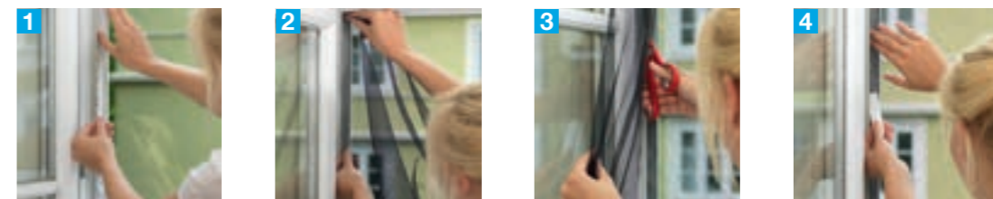
1 Attach Hook & Loop tape 2 Press the mesh onto the tape 3 Simply cut off excess length 4 Use fixing device for a perfect hold
